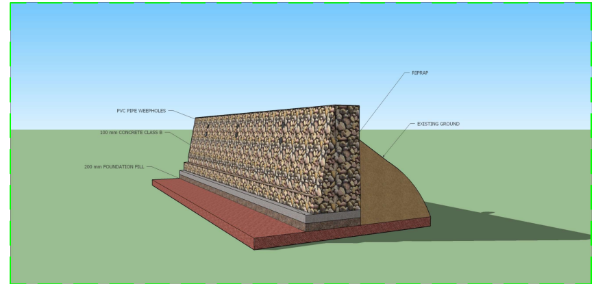
CONSTRUCTION OF RIPRAP ATLEAST 280 l.m. LENGTH
